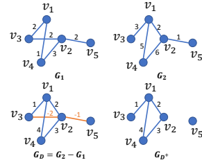
Fig. 1. An Example of the Difference Graph
