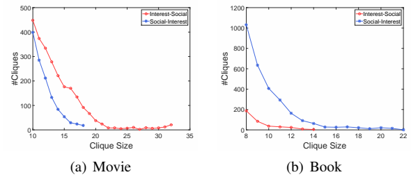
Fig. 3. Clique Counts of Douban Data
