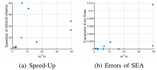
Fig. 2. SpeedUp of SEACD+Refine and Errors in Expansions of SEA+Refine
